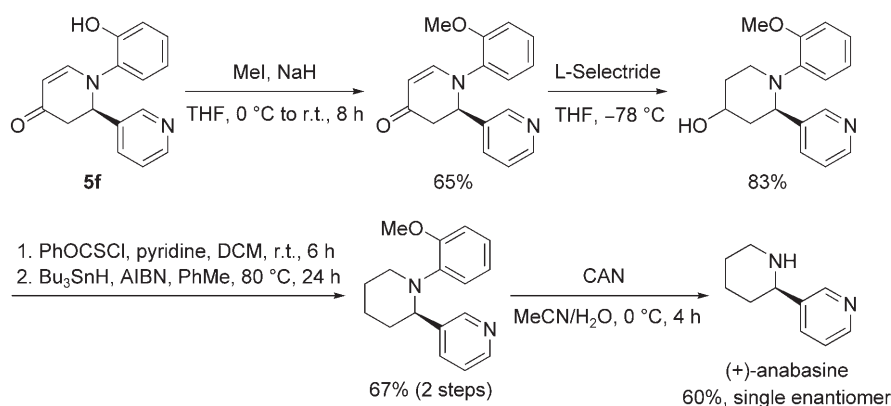
Scheme 1. Synthesis of (+)-anabasine.
