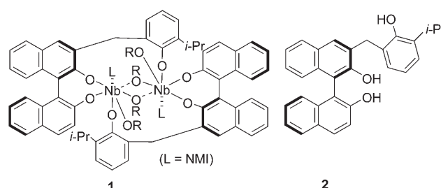
Figure 1. Tridentate ligand and proposed catalyst structure.
